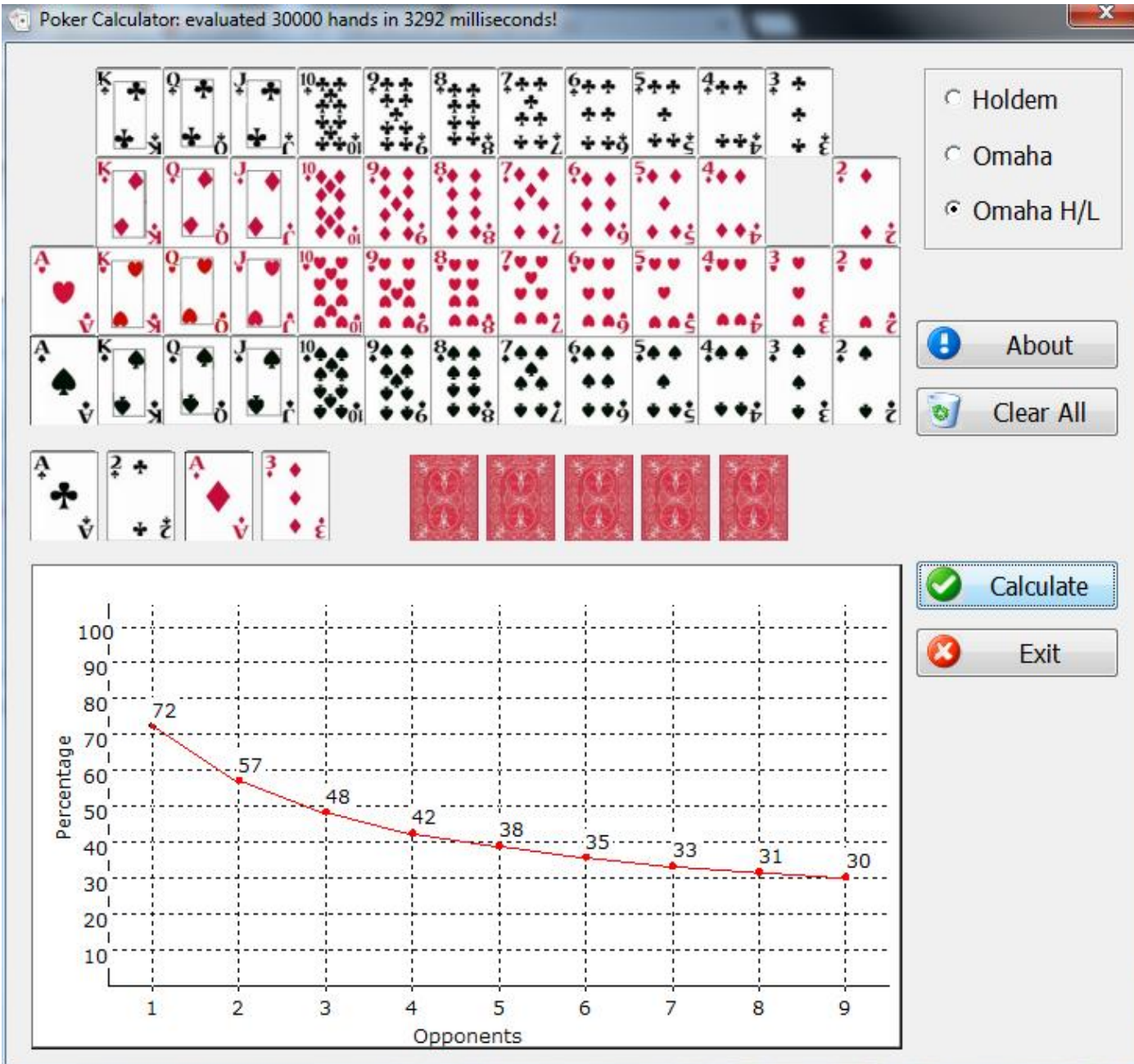
Fig.6 Result for strongest hand in Omaha Hi/Lo
