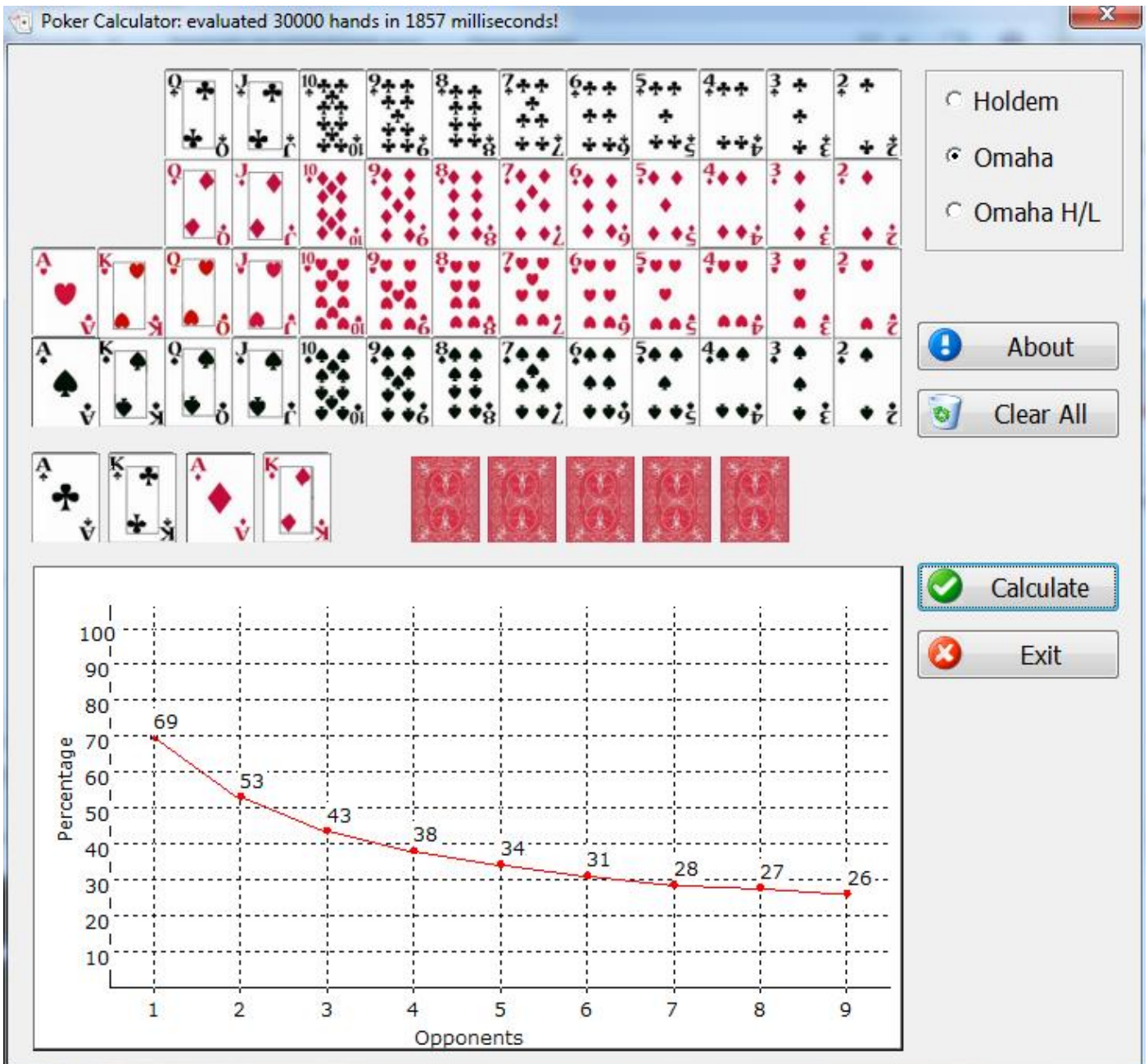
Fig.4 AcKcAdKd for Omaha
